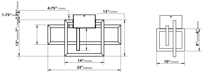
Overall Dimension : 600x254x375mm
