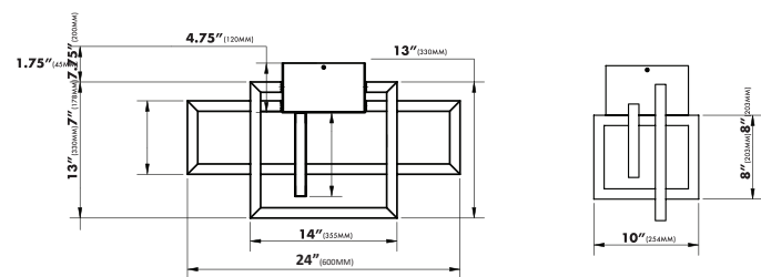
Overall Dimension : 600x254x375mm
