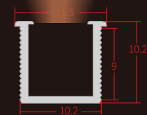
A-1010a Inside Cabinet Spotlight
