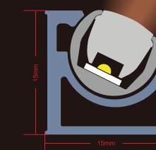
B Series | B-1515 Surface-mounted (Triangular Adjustable Angle)
