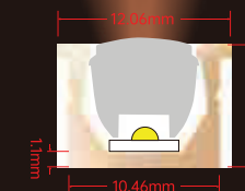
A-1010b Cabinet Side Light
