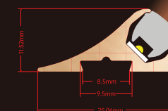
B-B2813 Adjustable Cabinet light
