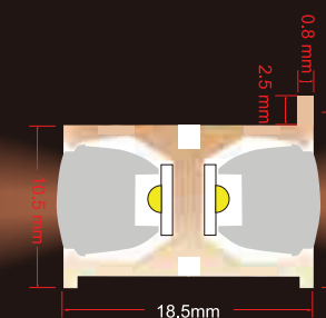
A-1119 Cabinet Back Light
